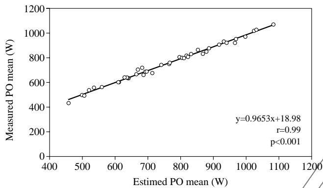
Figure 3.—Relationship between the SRM PO_{\text{mean}} measurement during sprints in the gymnasium and PO predicted by the mathematical model.
